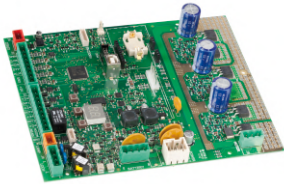
E680 electronic board
